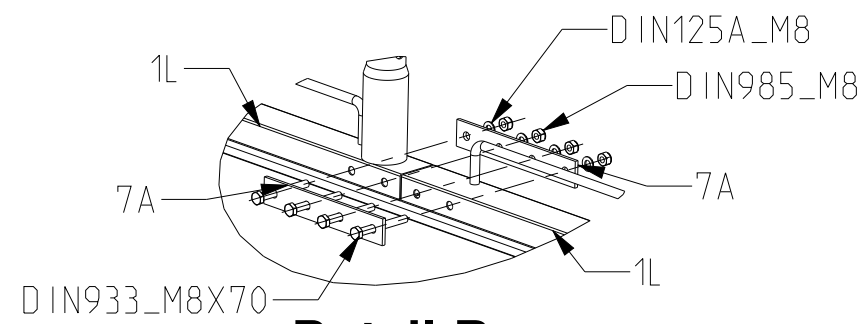
Detail B (1:8)
