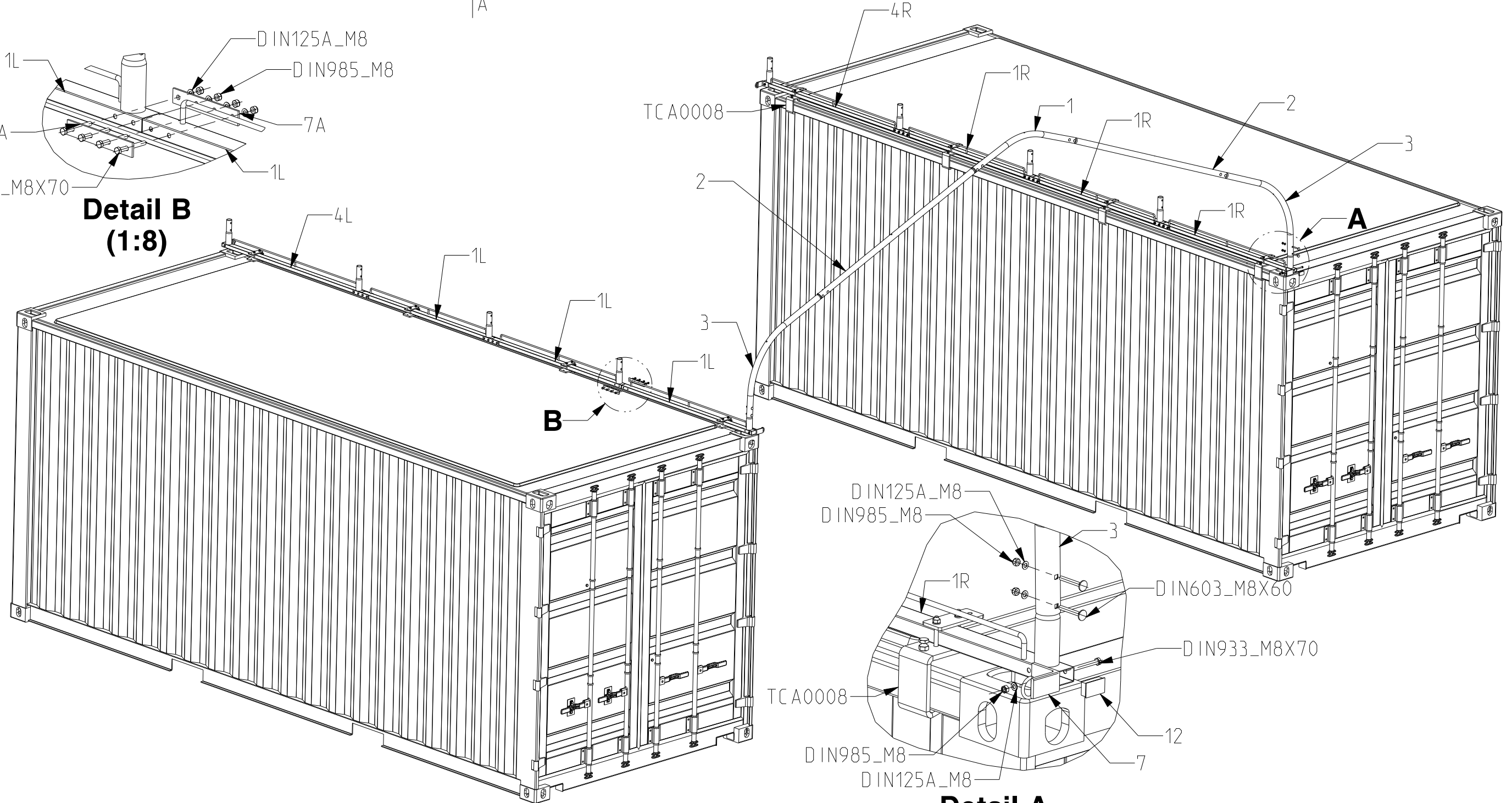
Detail A (1:8)
